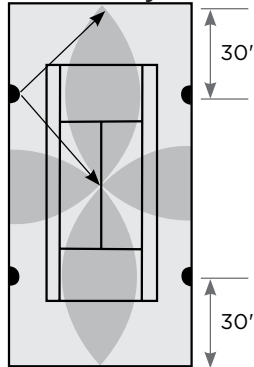
4-Head Layout
