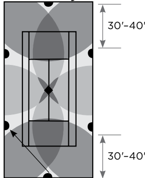
6-Head Layout
