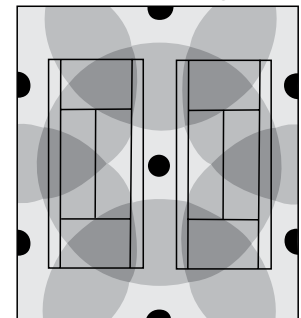
Battery of Two Courts 7- Or 8-Head Layout
